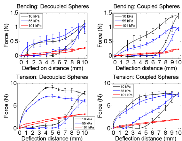
Figure 2. Results of jamming coupled and decoupled granules at atmospheric, mid, and full vacuum.
